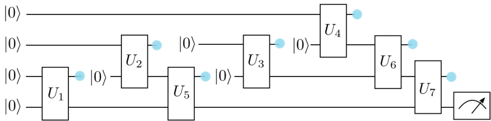
Resets + Measurements to Save Resources in NISQ machines
