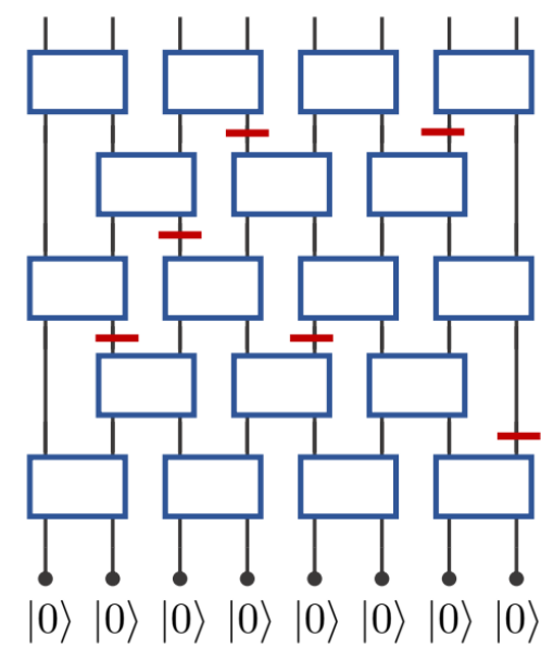
Measurement induced Phase Transition
